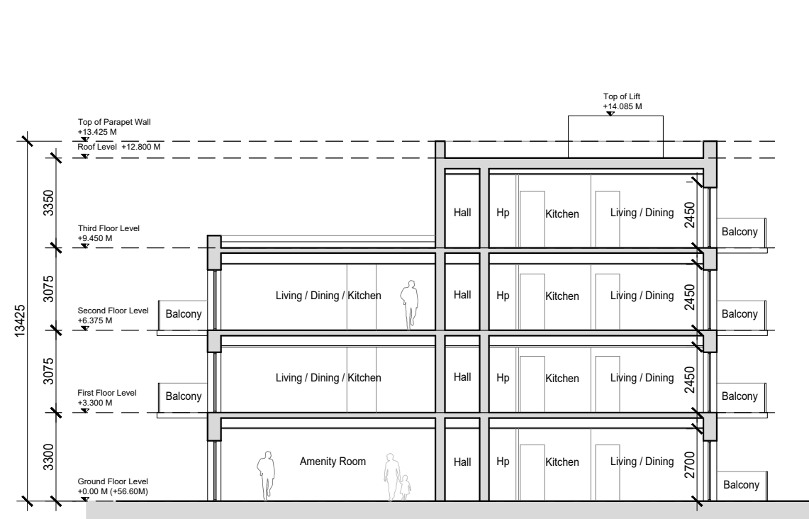
Block C - Section
