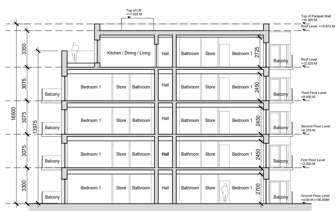
Block B - Section
