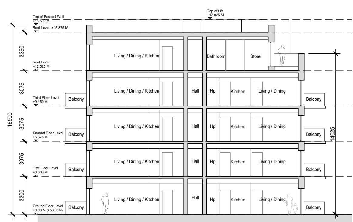
Block A - Section
